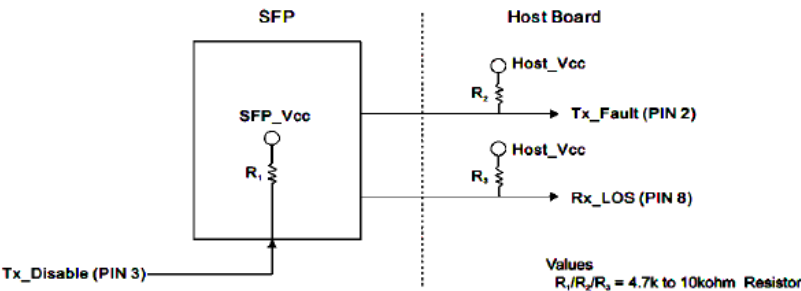
Figure 2. Signal Definitions
