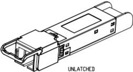
UNLATCHED
